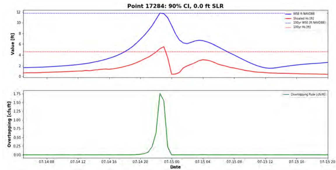
Figure 4. Timeseries of water surface elevation and wave heights (top) compared to overtopping rates (bottom).
