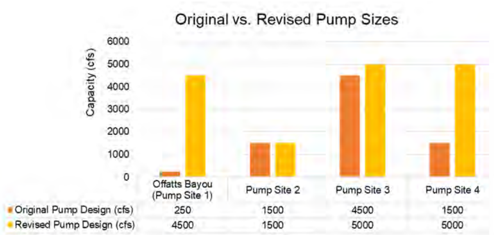
Figure 14. Comparison of original (orange) and revised (yellow) designed pump size capacities.
